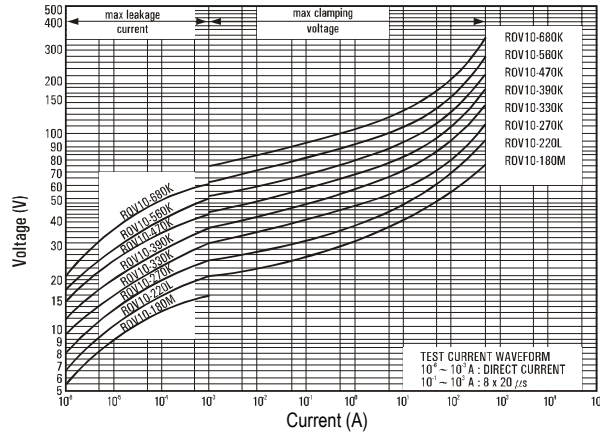
ROV10-180M – ROV10-680K
