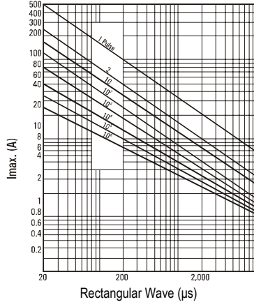
ROV10-180M – ROV10-680K
