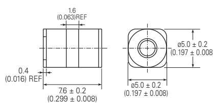
Surface-mount (GTCS35-XXXM-R05)
