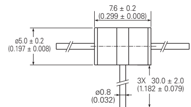
T Leaded (GTCT35-XXXM-R05)
