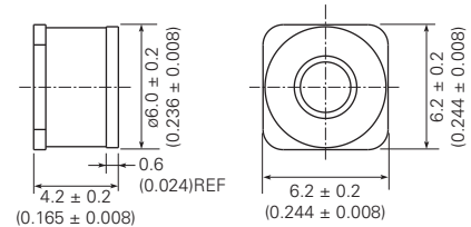
Surface-mount (GTCS26-XXXM-R05)
