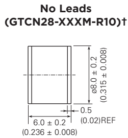
Figure G6 Two Electrode 8mm Product Dimensions
