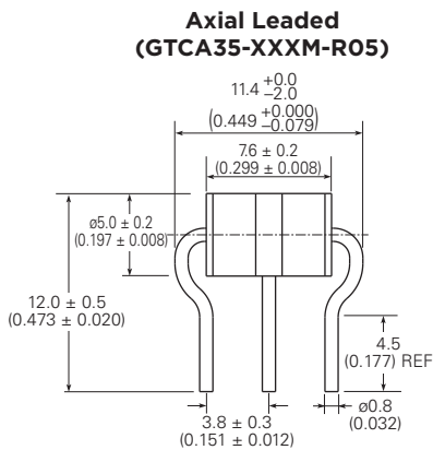
Figure G7 Three Electrode 5mm Product Dimensions
