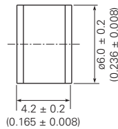
No Leads (GTCA26-XXXM-R05)†
