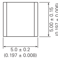
No Leads (GTCA25-XXXM-R02)†
