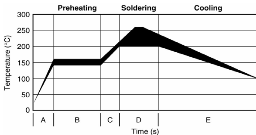
FIGURE 3. REFLOW PROFILE
