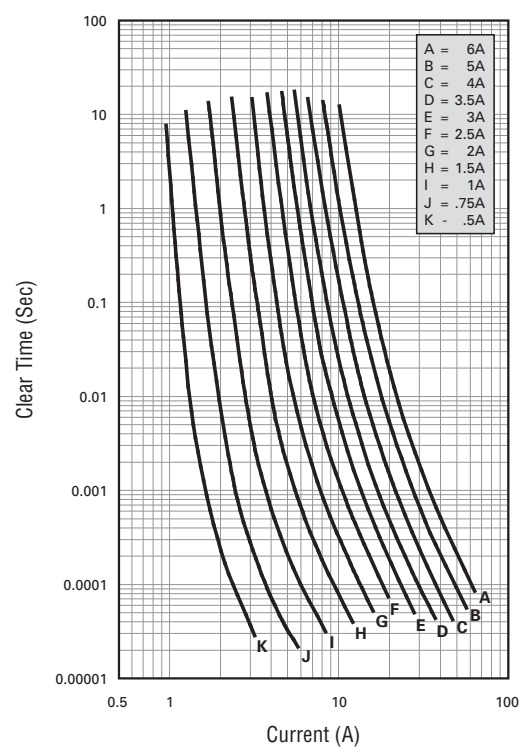
Figure FF3 - 0603SFF Family Average Clear Time
