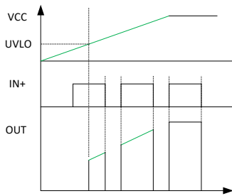
MX27517 start up waveform
