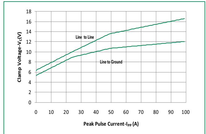
Figure 4: Clamp Voltage vs. Peak Pulse Current
