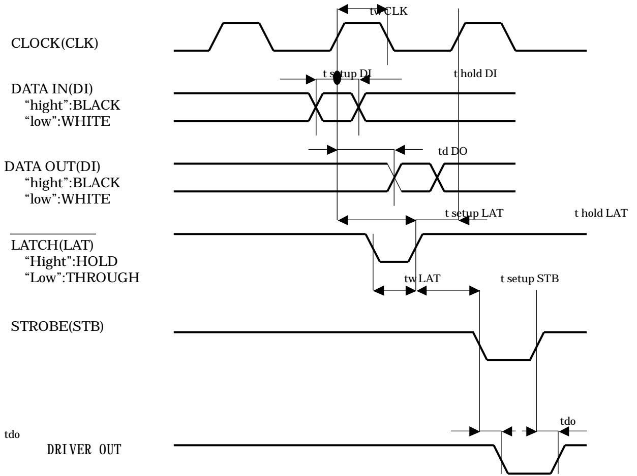
Figure 3-1 Timing chart
