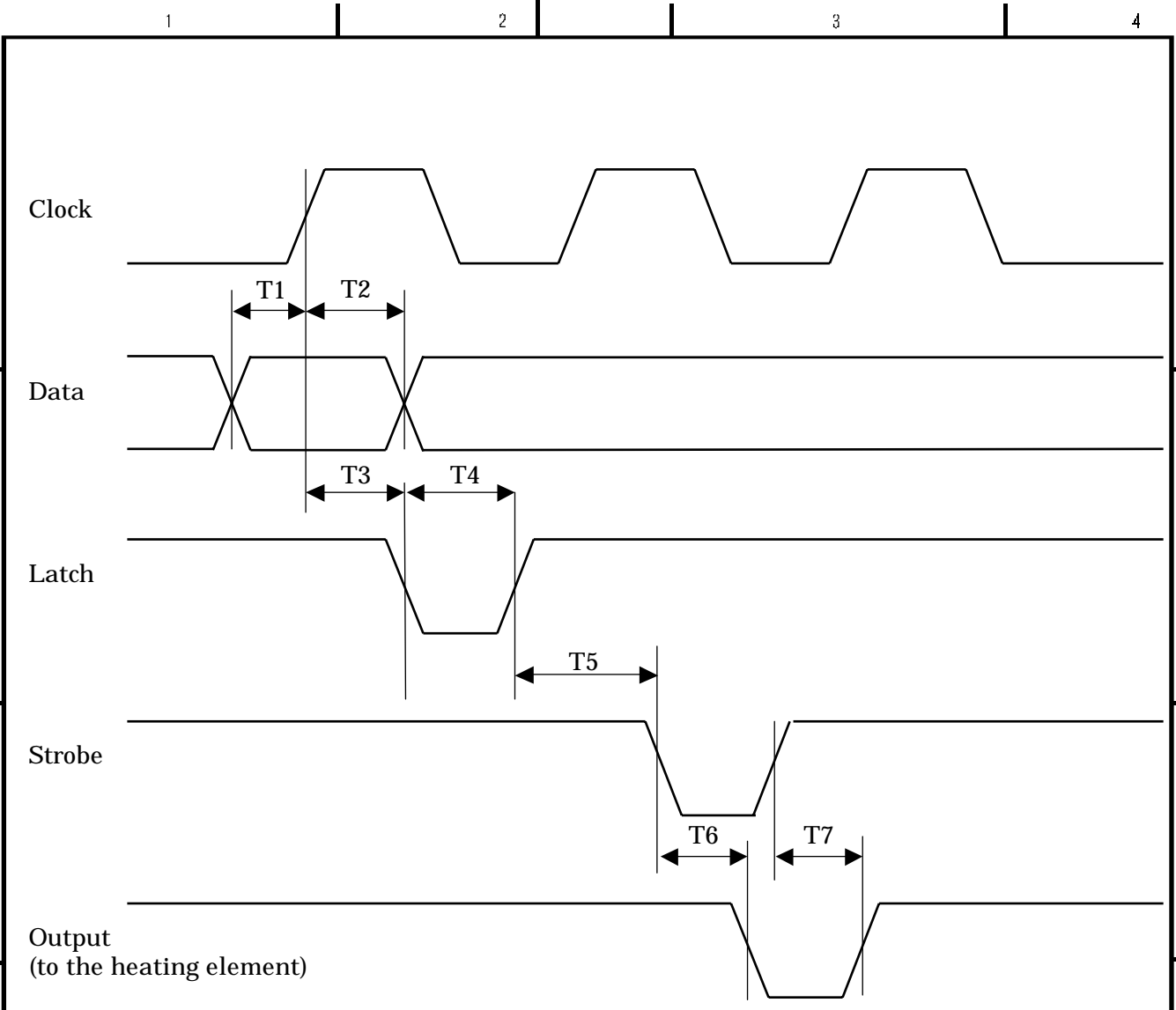
Figure 5 Timing chart
