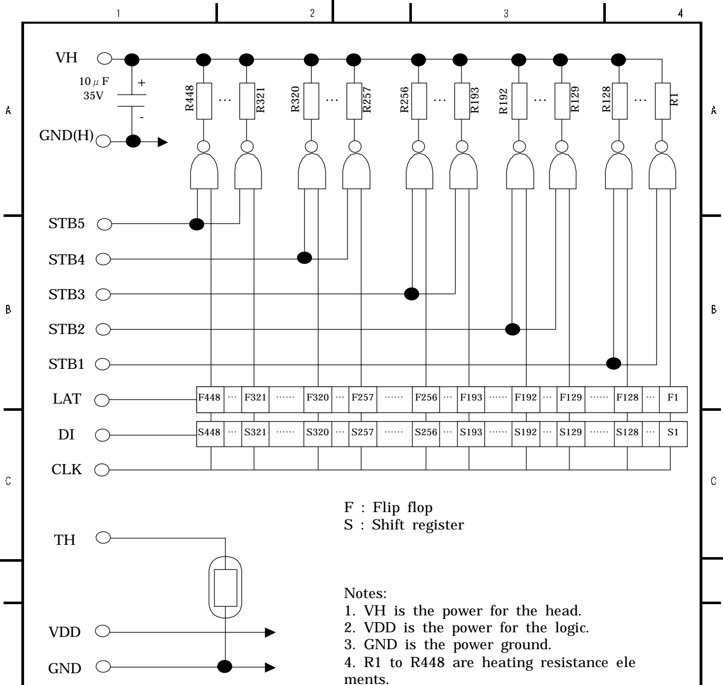
Figure 6 Electric circuit block diagram
