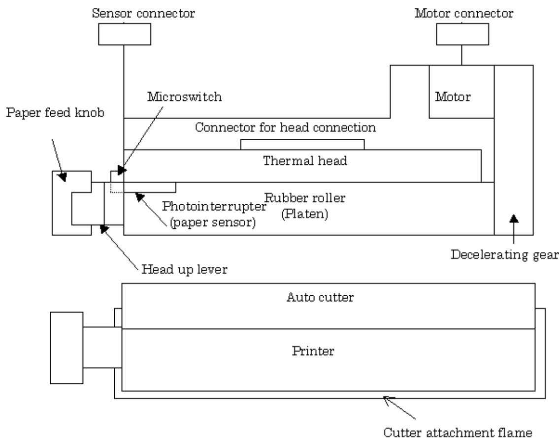
Figure 1 Printer configuration
