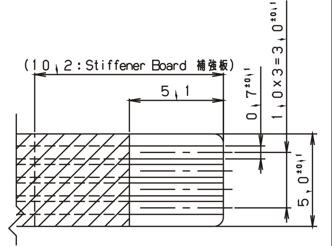
Conductive Face (導通面) FFC-Type Cable
