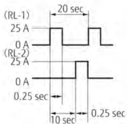
Current wave form
