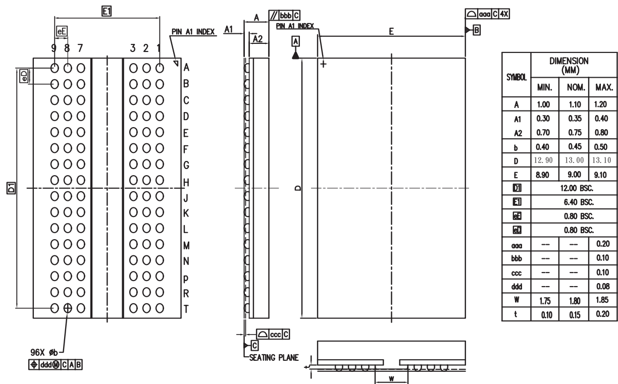
96-Ball Fine Pitch Ball Grid Array Outline
